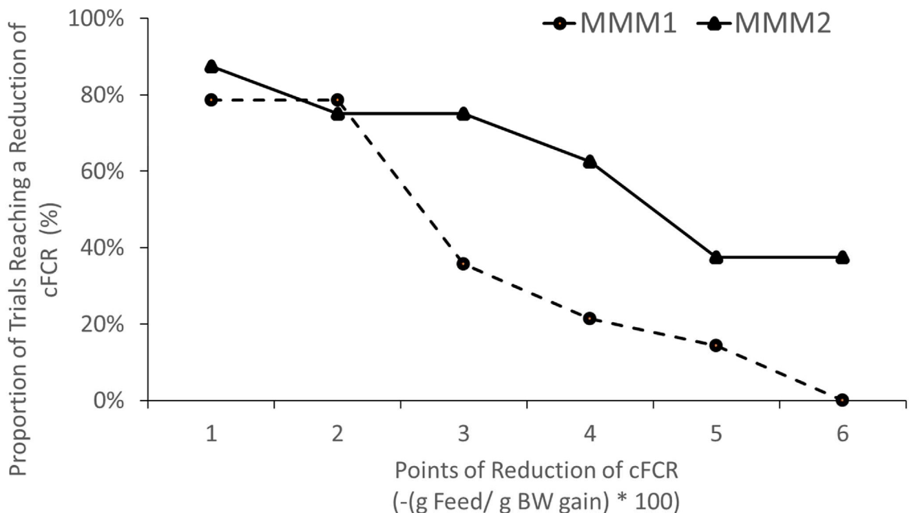
Figure 1. Percentage of broiler chicken trials reaching different levels of the cFCR (mortality and BW-corrected FCR) for 2 distinct microbiome metabolic modulator products (MMM1 and MMM2) applied in feed at 500 g/MT.
