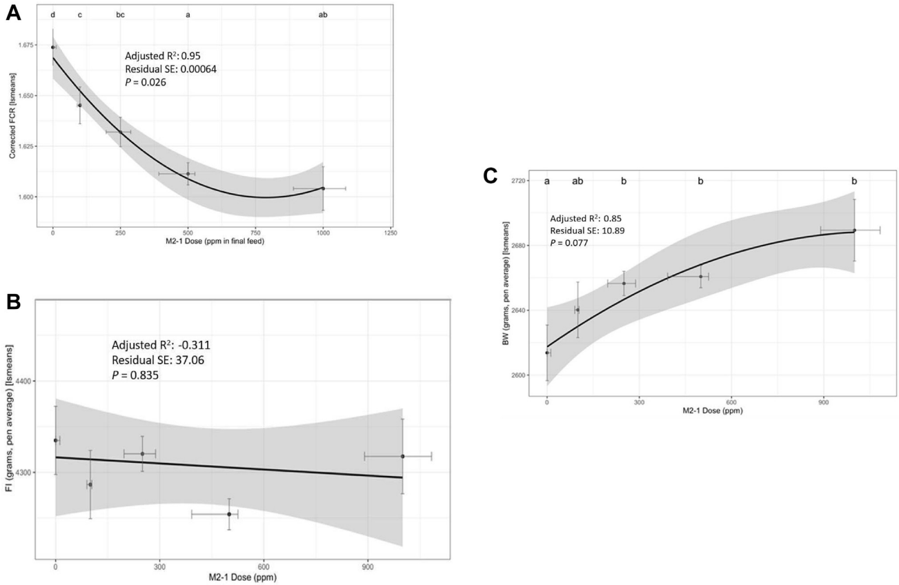
Figure 2. Tukey’s corrected Ls mean comparisons and smooth regressions of the effect of dose in feed of microbiome metabolic modulator MMM2 (M2-1) on (A) the BW and mortality-corrected FCR (cFCR); (B) cumulative feed intake, and (C) the final BW in 8 trials with broiler chickens from 0 to 32-42 days. Vertical error bars reflect the SE in the mean. Horizontal error bars reflect the estimated range of doses formulated into feed for each intended dose level. Inclusion of the glycan microbiome metabolic modulator (MMM2) in the final feed was determined by liquid chromatography with tandem mass spectrometry (LC-MS/MS) using methods described previously (Geremia et al., 2020b). For each dose level, the error bars were determined as the (asymmetric) 1-sigma CI obtained from in-feed assaying of pelleted samples drawn from n = 35 independent diet formulations (i.e., study, treatment group, and phase). a-d Means with different superscripts differed at P < 0.05.
