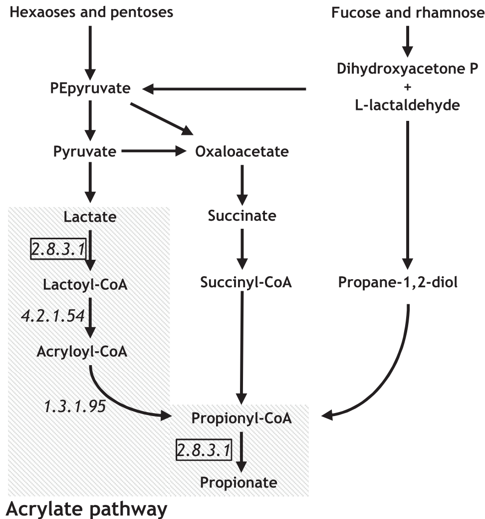
Figure 3. Schematic representation of the known pathways for propionate formation in gut bacteria (based on the study by Reichardt et al., 2014), with emphasis on the acrylate pathway, highlighted in gray.
