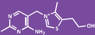
Molecular formula of thiamine
