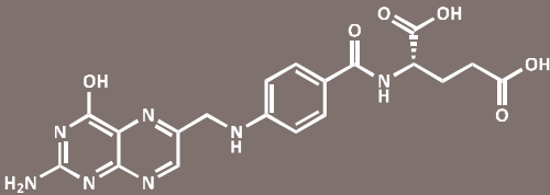
Molecular formula of folic acid
