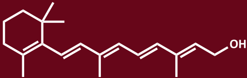
Molecular formula of vitamin A (retinol)
