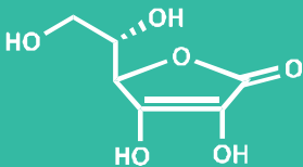
Molecular formula of vitamin C
