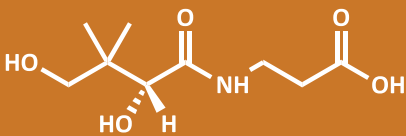
Molecular formula of pantothenic acid
