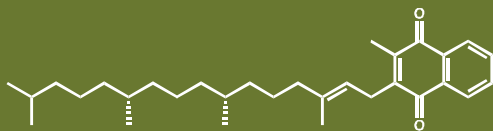
Molecular formula of vitamin K
