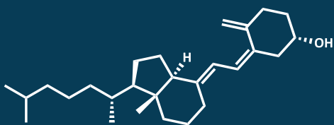
Molecular formula of vitamin D
