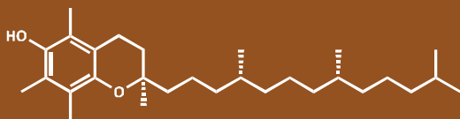
Molecular formula of vitamin E
