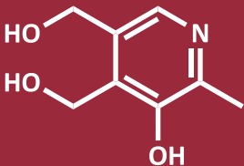
Molecular formula of vitamin B6
