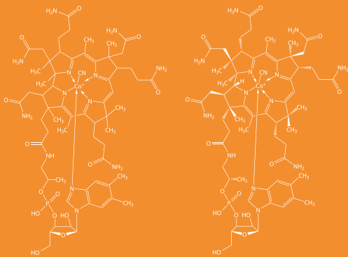
Molecular formula of vitamin B12
