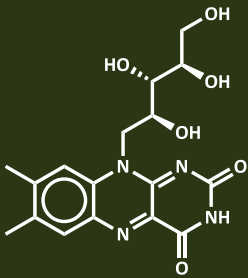
Molecular formula of riboflavin
