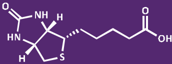
Molecular formula of biotin
